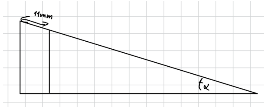
Figure 4.3: Schematic representation of the height difference h and the length of the ramp L .
