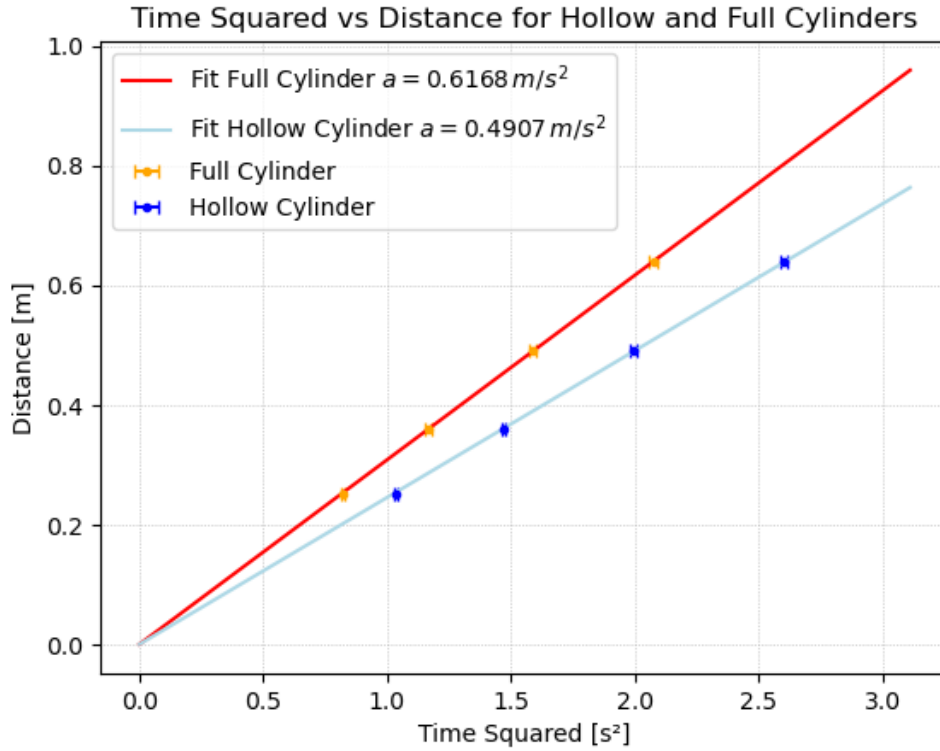
Figure 4.2: Comparison of theoretical and experimental accelerations for solid and hollow cylinders.
